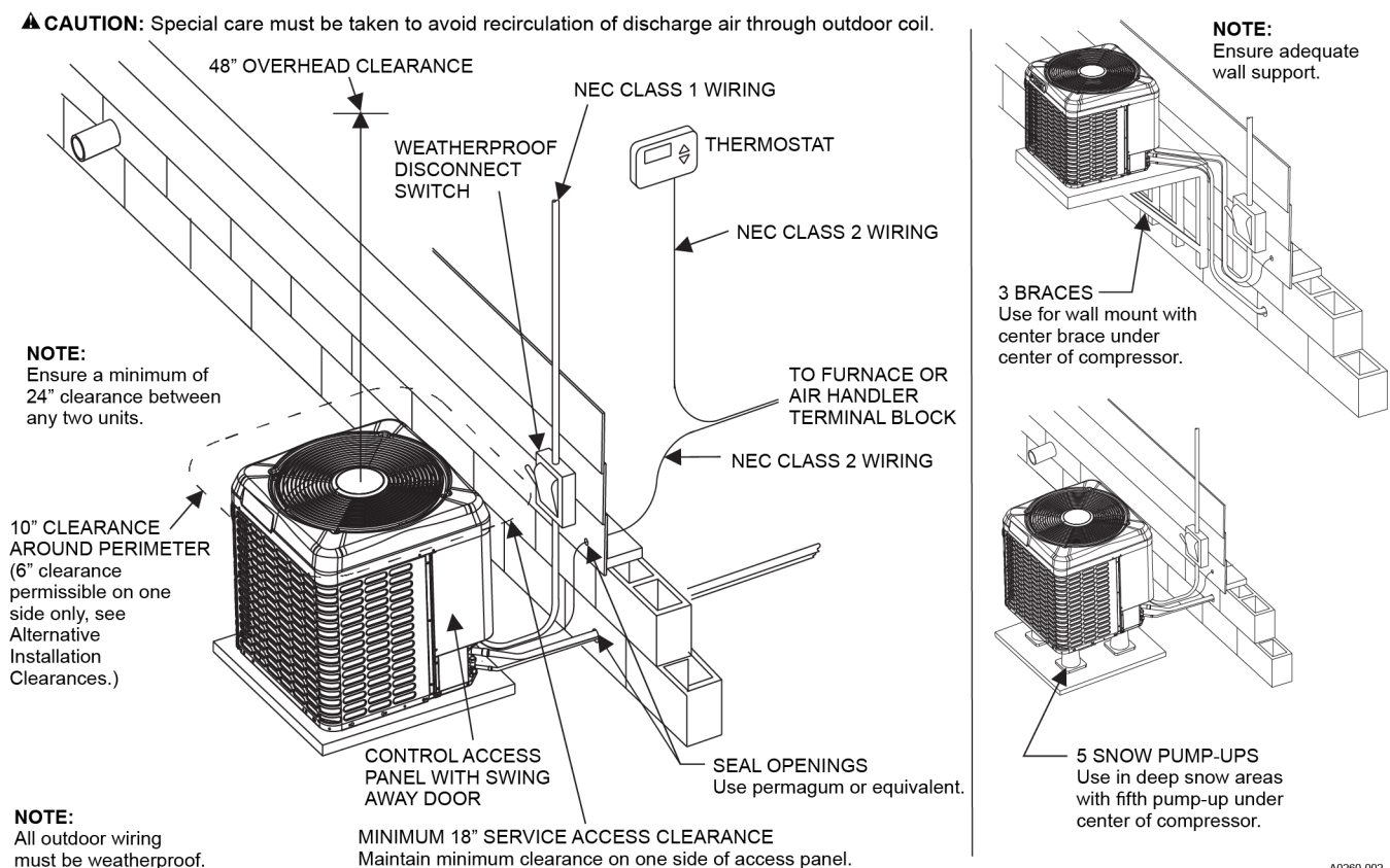
Figure 3: Typical installation
